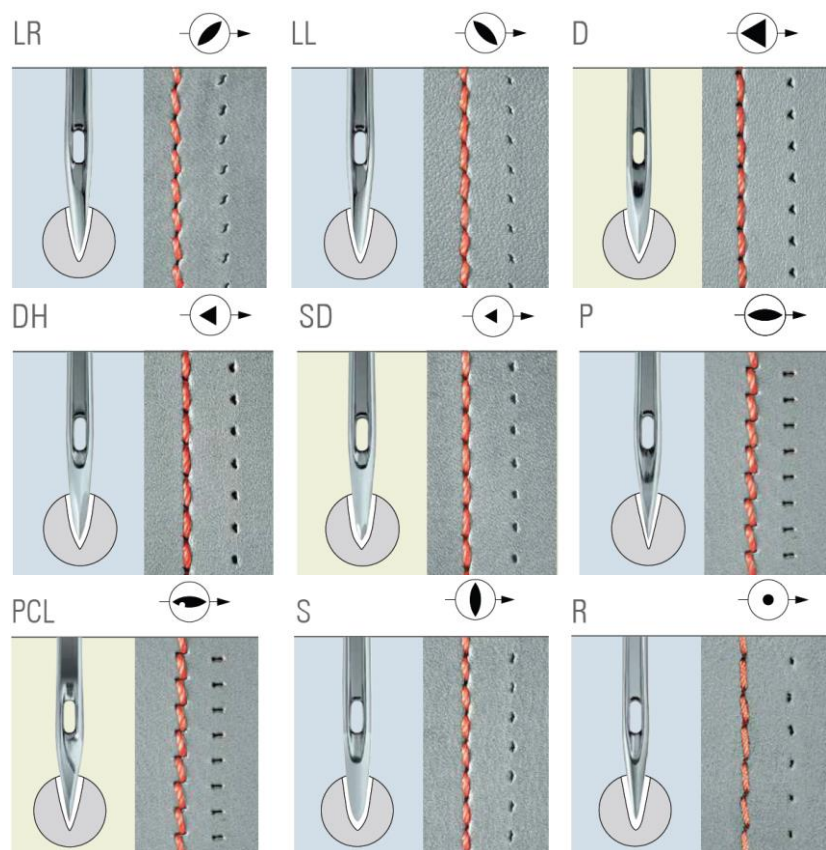
Fig.9 Shape of blades of machine sewing needles for sewing leather according to tt. Groz Beckert [7]
