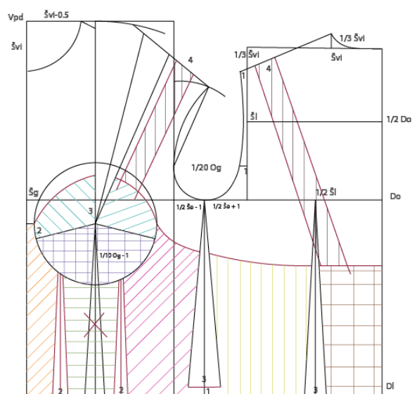
Fig.13 Corset construction and modeling [27]
