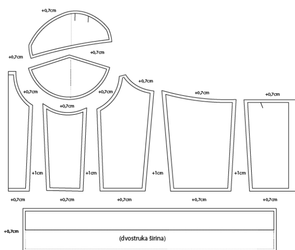
Fig.15 Pattern parts of basic fabric for corset [27]
