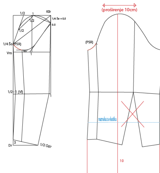
Fig.14 Sleeve construction and modeling [27]
