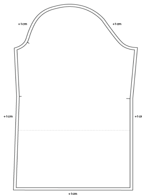
Fig.16 Sleeve pattern part with seam allowances [27]
