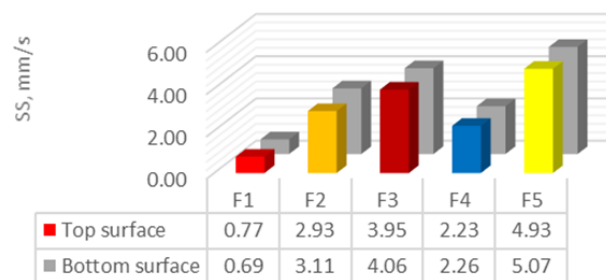
Fig.8 Spreading speed (SS) on tested knitted fabrics
